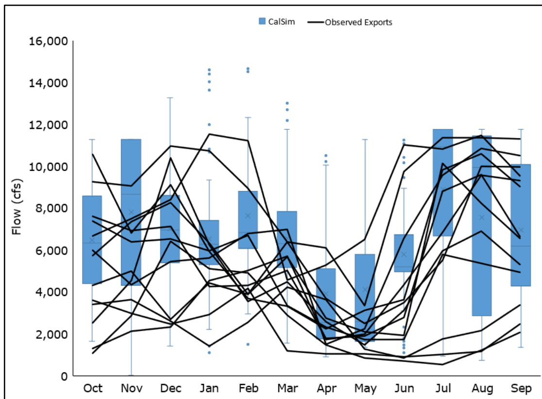
Figure 4-4. Total Delta Exports, Historical and Modeled Baseline Conditions
