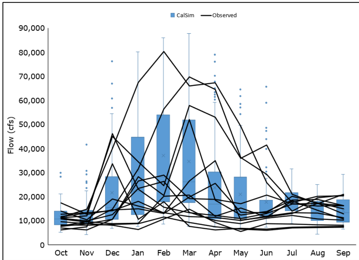
Figure 4-2. Sacramento River at Freeport, Historical and Modeled Baseline Conditions Flow
