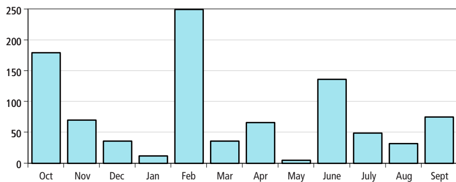
Number of Statewide Precipitation Records by Month for Water Year 2015
