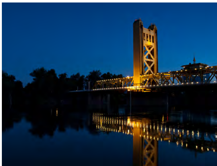
The Sacramento Valley 40-30-30 Index based on flow in million acre feet for water year 2016 was 84 percent of average with an index value of 6.7 classified as a "below normal" water year type.
