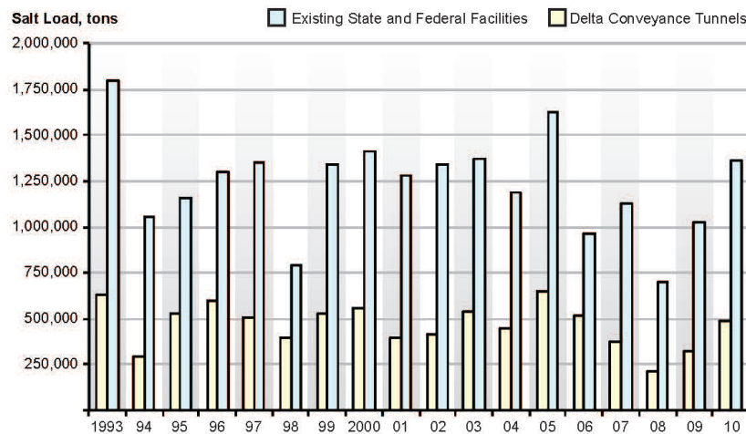
Figure 2 Salt Loads Comparison: Existing South Delta State and Federal Pumping Plant Intakes vs. Proposed Delta Conveyance Tunnel
