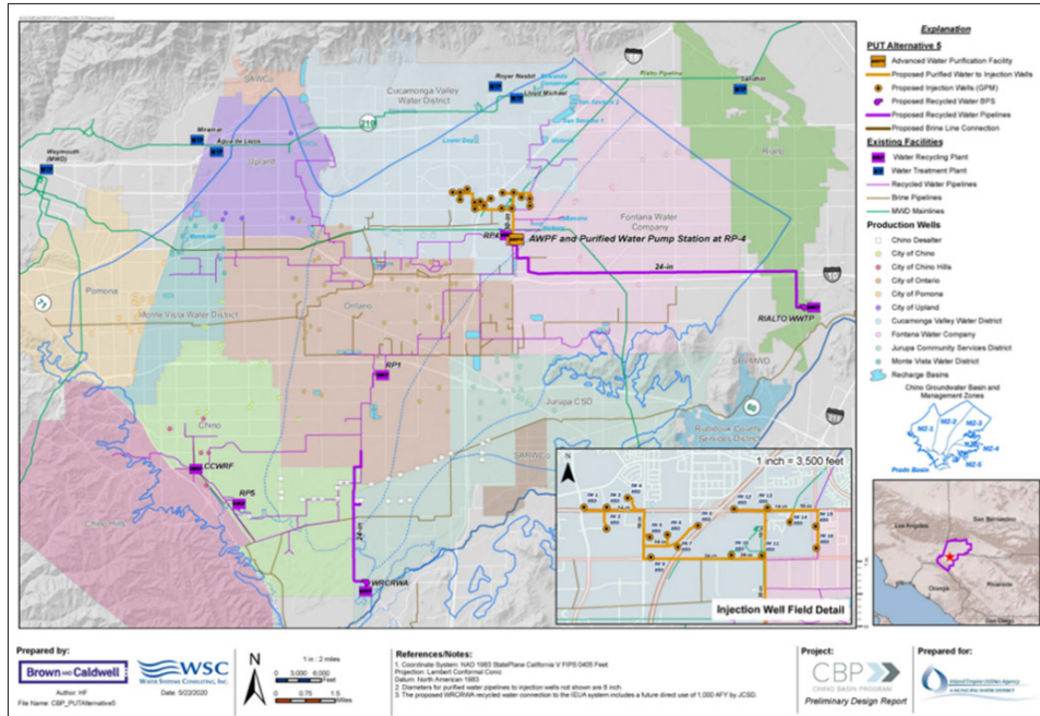
Figure 2-2a. Preferred Configuration of CBP PUT Facilities
