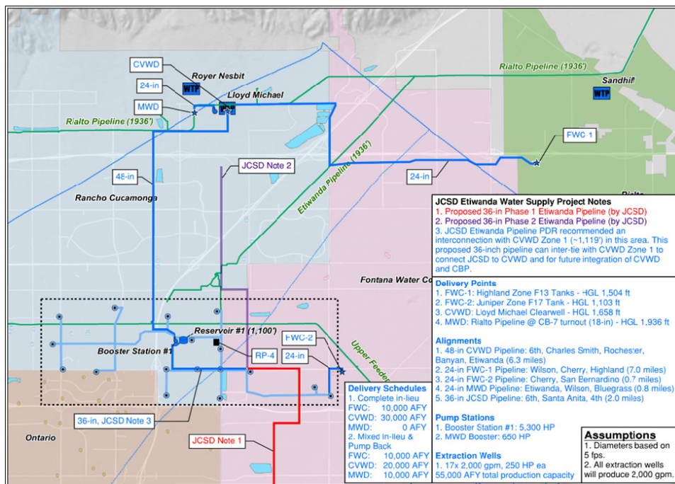
Figure 2-3b. Preferred Configuration of CBP TAKE Facilities
